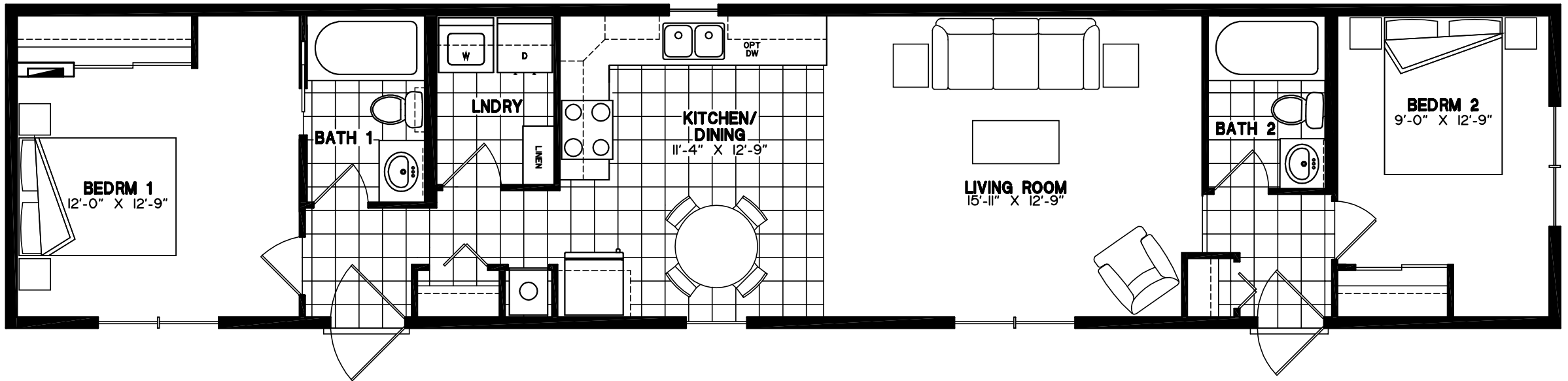
16-4454 66'x14' Mobile Home (907sq.ft.)
