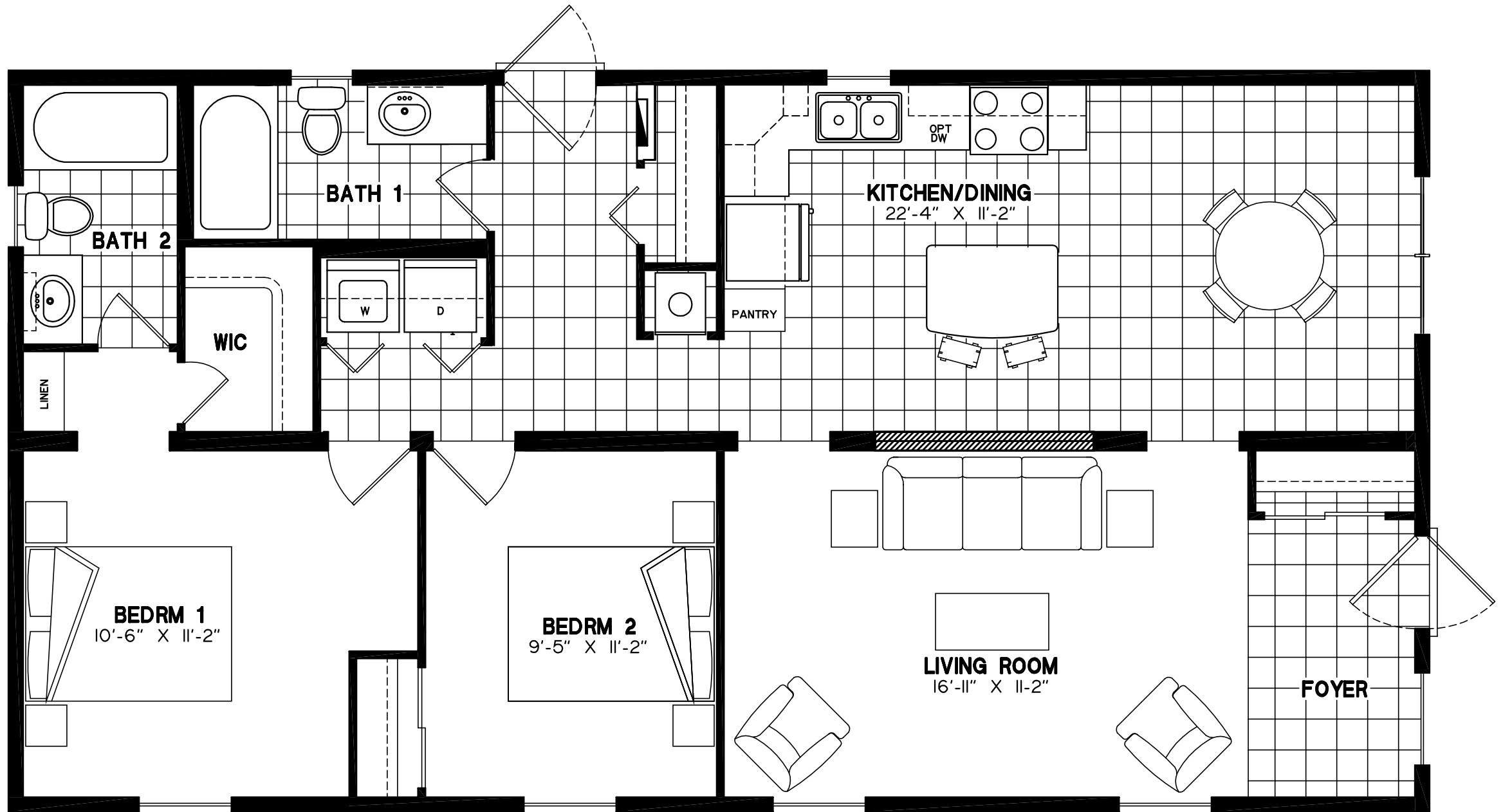
ASPIRE MODULAR 4624-003 (1104 sq.ft.)
