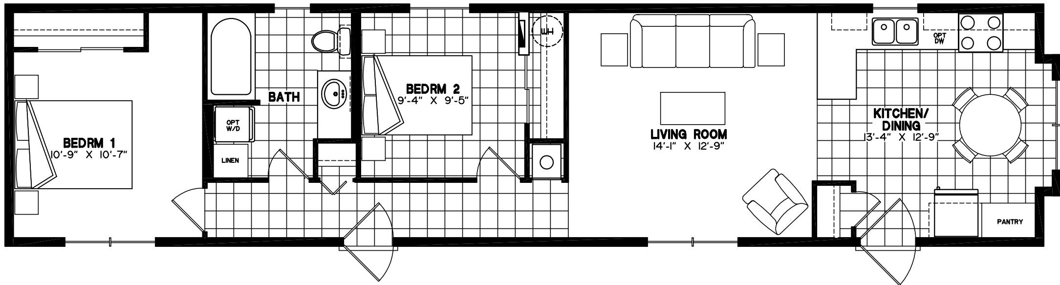
16-4450 60' x 14' Mobile Home (825sq.ft.)
