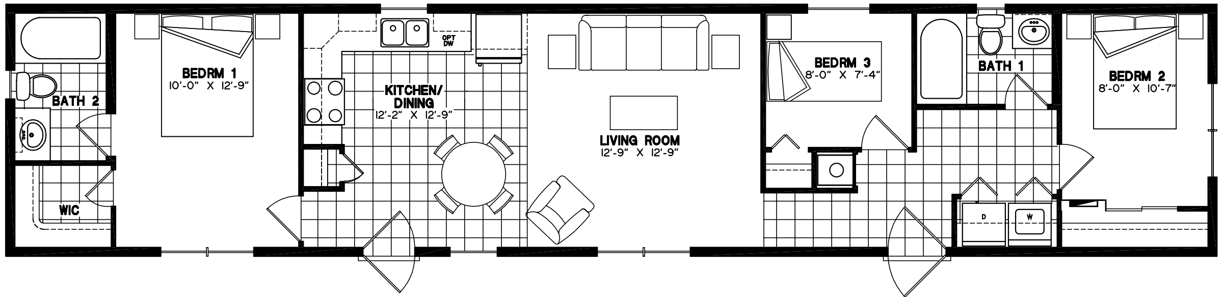
16-4455 66' x 14' Mobile Home (907sq.ft.)
