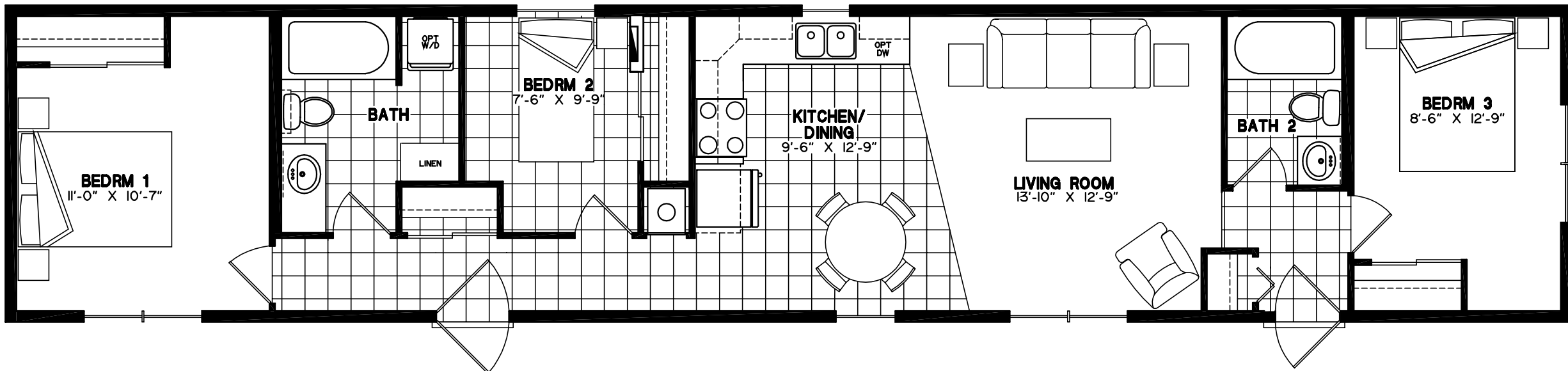
16-4457 68' x 14' Mobile Home (935sq.ft.)
