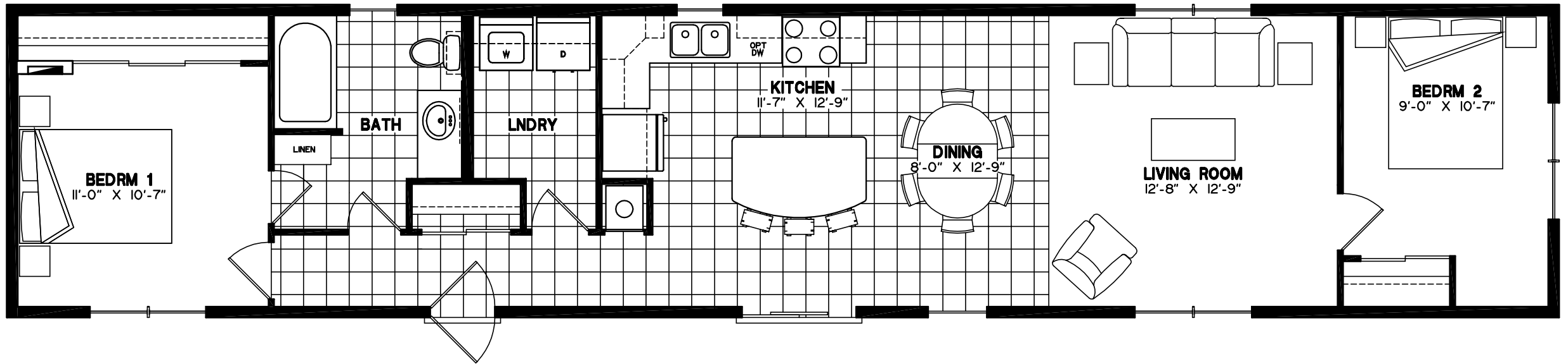
16-4458 68' x 14' Mobile Home (935sq.ft.)
