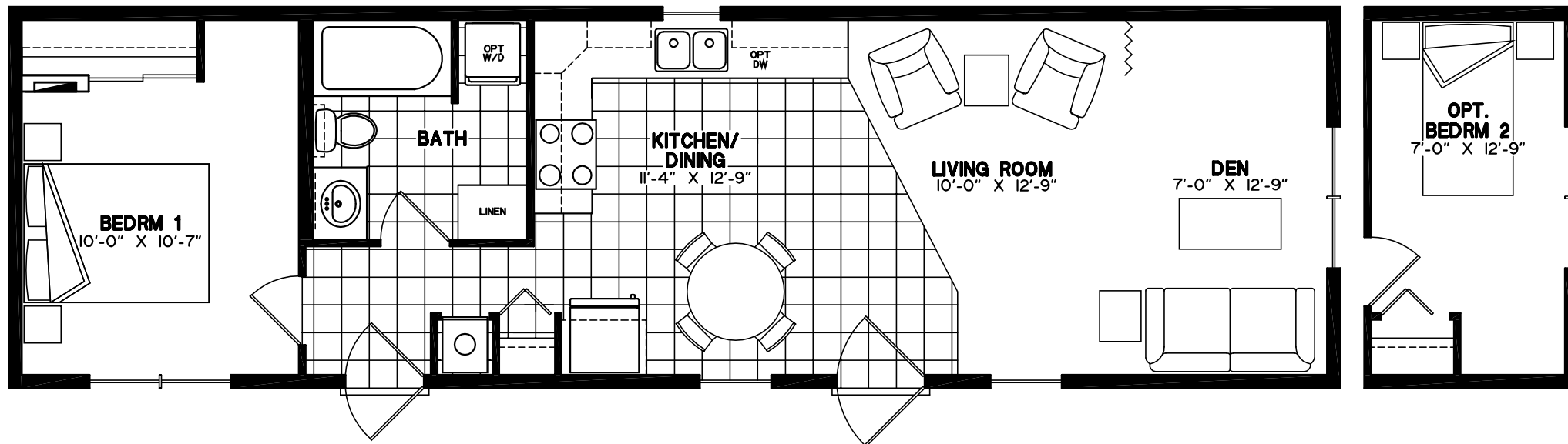
16-4446 48' x 14' Mobile Home (660sq.ft.)
