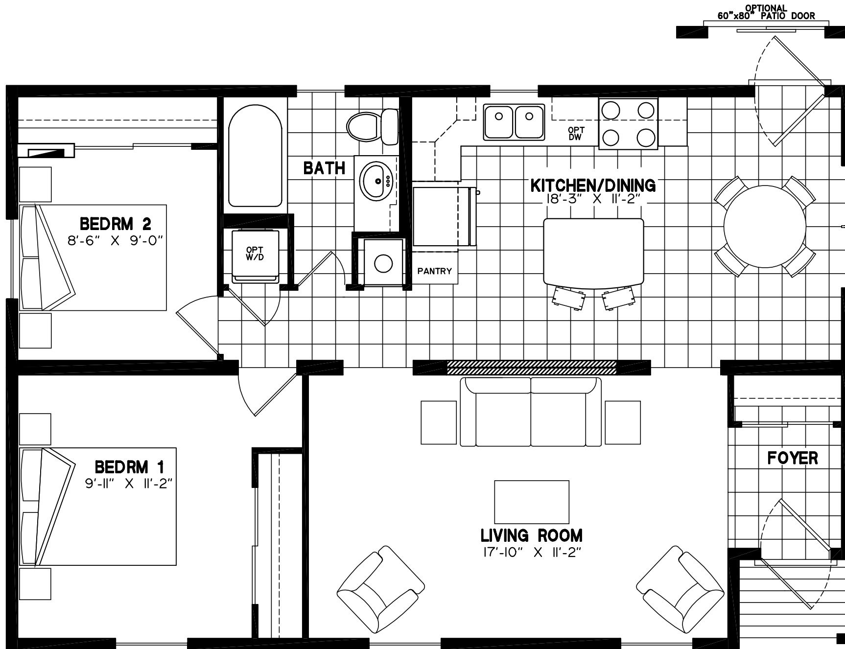
ASPIRE MODULAR 3624-001 (846 sq.ft.)
