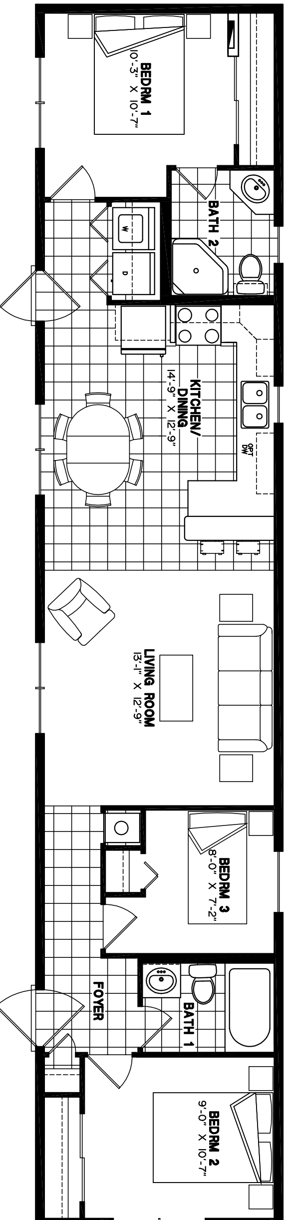
16-4456 68' x 14' Mobile Home (935sq.ft.)
