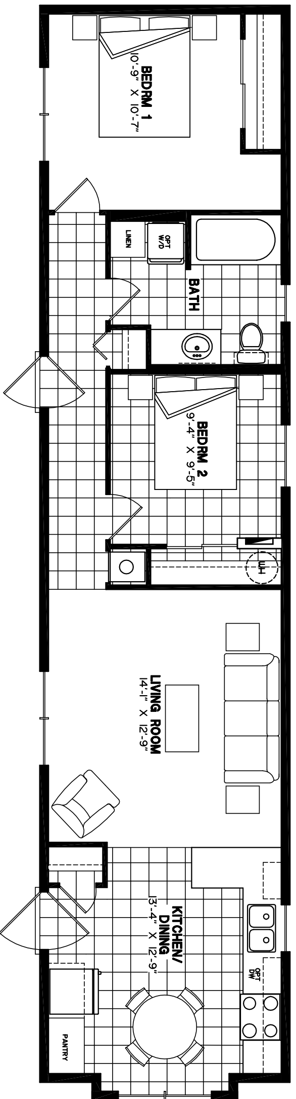
16-4450 60' x 14' Mobile Home (825sq.ft.)
