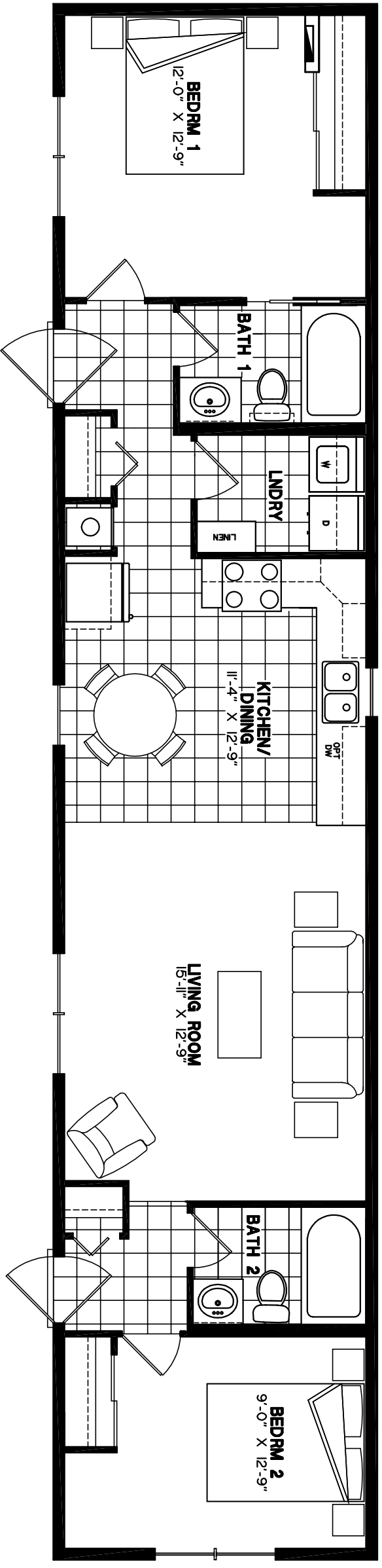
16-4454 66' x 14' Mobile Home (907sq.ft.)
