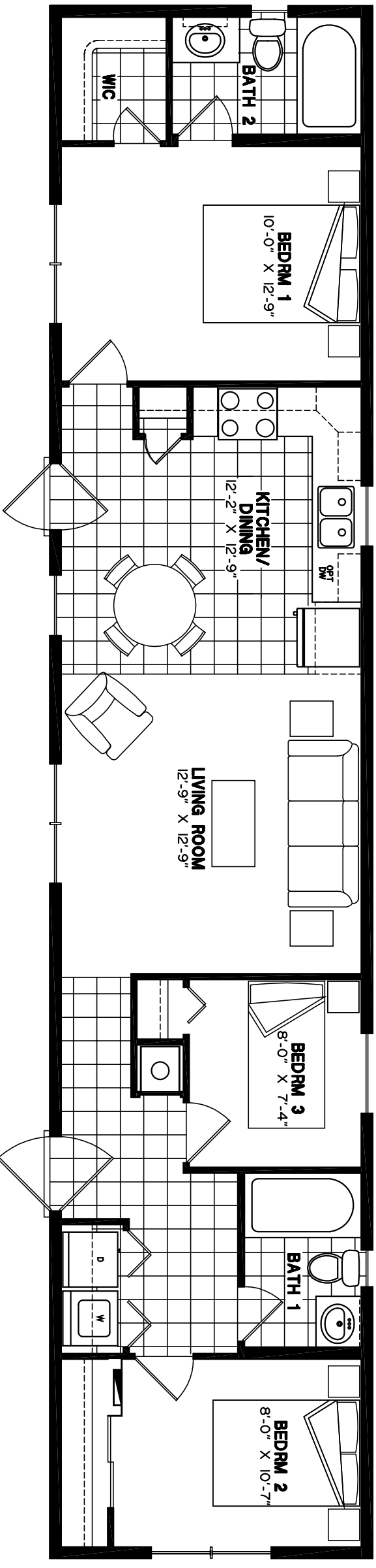
16-4455 66' x 14' Mobile Home (907sq.ft.)
