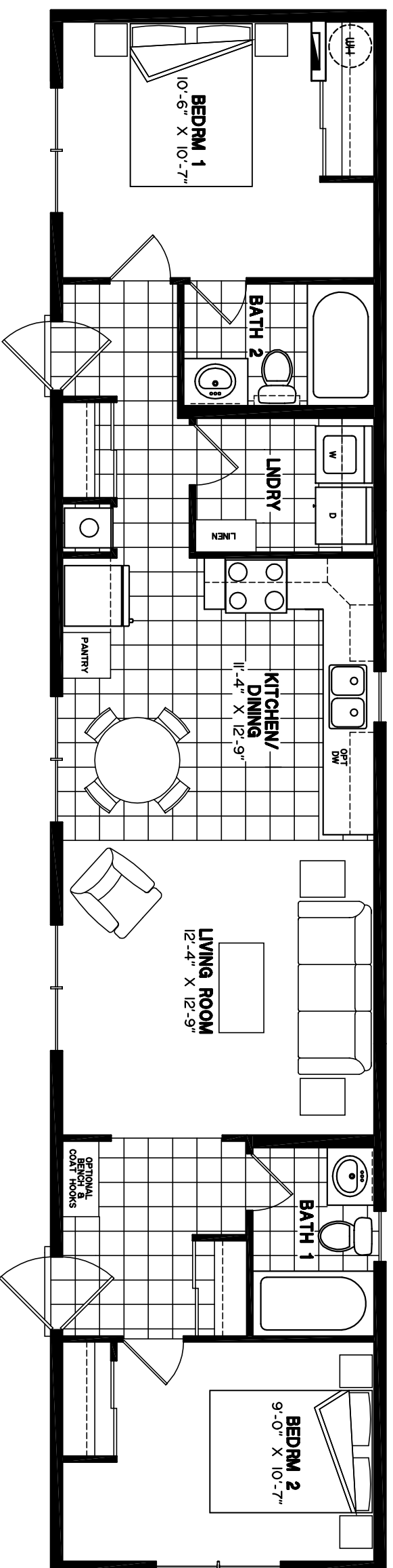
16-4452 64' x 14' Mobile Home (880sq.ft.)
