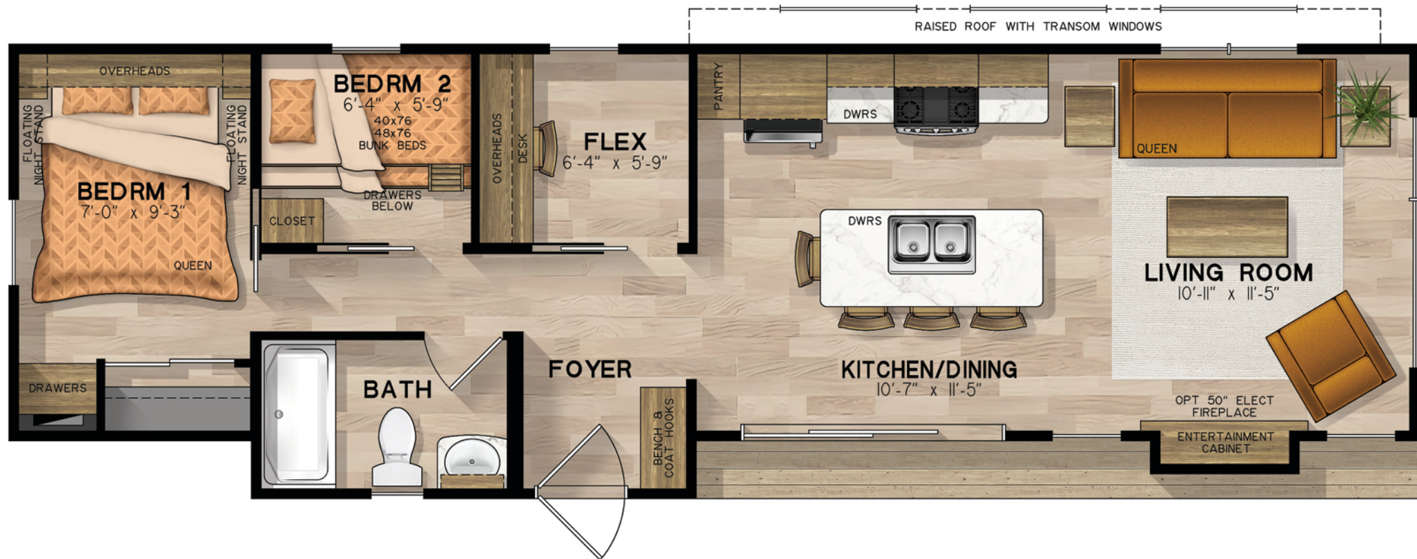
Elrose 25-5247-2TR 42'-7" x 13'-9" Escape (539sq.ft.)
