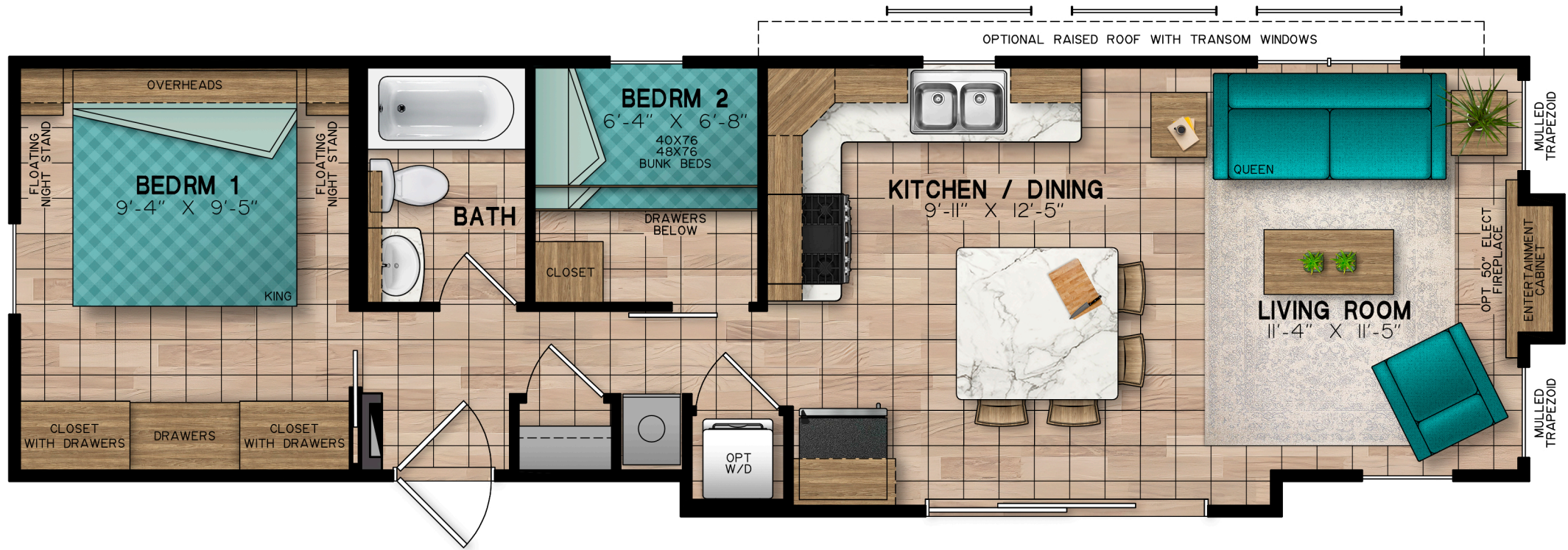
Atlanta 23-4999-2 43' x 12' All Season (537sq.ft.)
